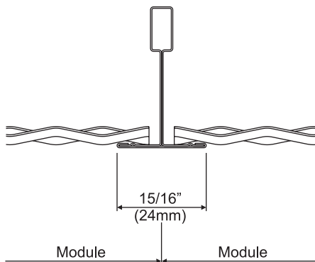
Fig. 120 With lay-in type plate
