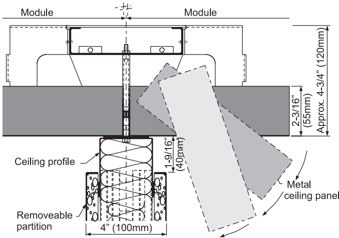
Fig. 57 Fold-down / hook-on system With horizontal longitudinal sound reduction, D_{n,f,w,P} = 42 \text{ dB}
