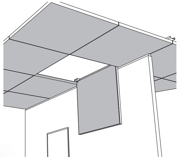
Fig. 57 Fold-down / hook-on system With horizontal longitudinal sound reduction, D_{n,f,w,P} = 42 \text{ dB}
