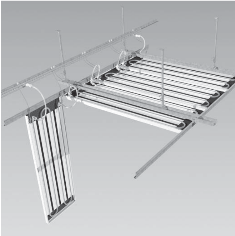
Fig. 12 Detail of Hook-On Ceiling, LMD Plafotherm E
