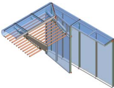
Use of 3D planning with complex facade design
