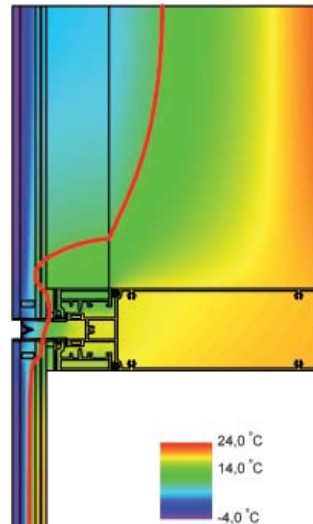
Energy testing of a facade system by means of isotherm calculations
